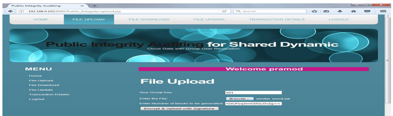
Fig5. File upload
