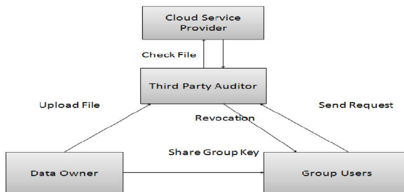
Fig1. System Architecture.
