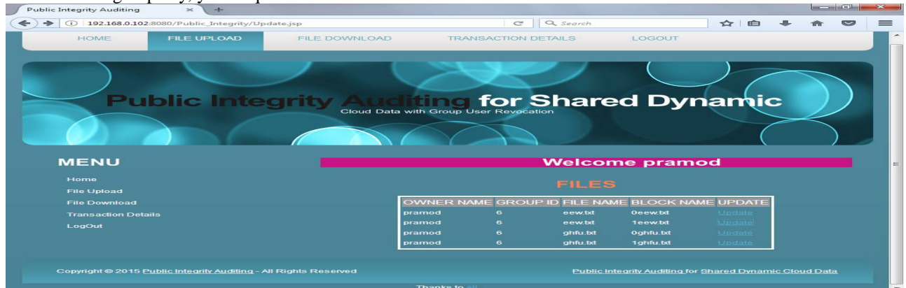
Fig7. File Update
